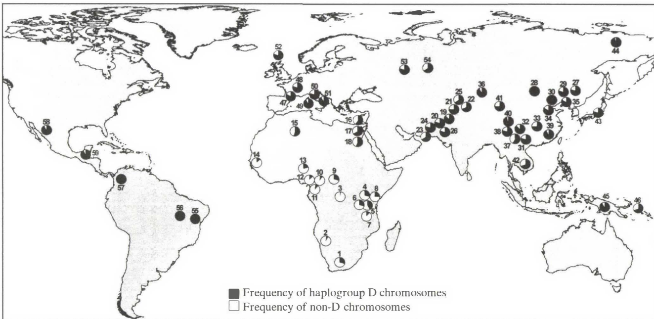
Fig. 3.1 Global frequencies of microcephalin haplogroup D chromosomes (defined as having the derived C allele at the G37995C diagnostic SNP) in a panel of 1184 individuals.
