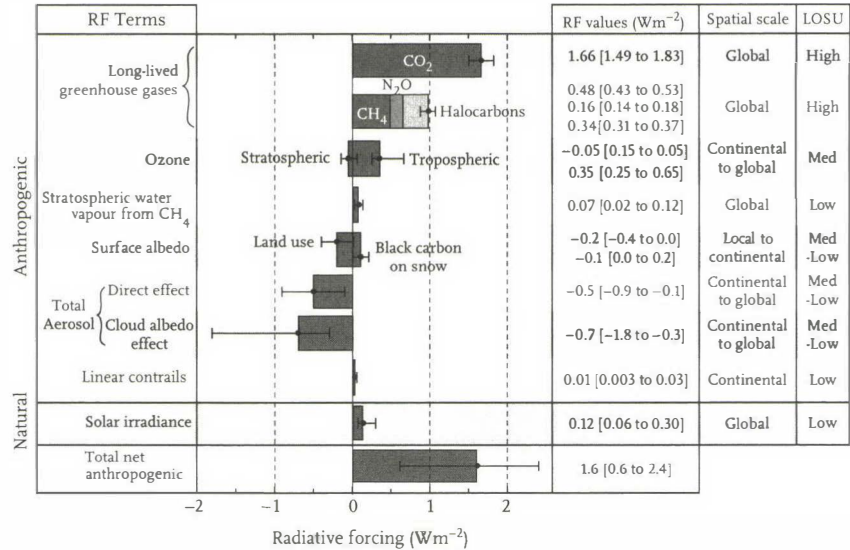
Fig. 13.1 Global average radiative forcing (RF) estimates and ranges in 2005 for anthropogenic carbon dioxide ( \text{CO}_2 ), methane ( \text{CH}_4 ), nitrous oxide ( \text{N}_2\text{O} ), and other important agents and mechanisms, together with the typical geographical extent (spatial scale) of the forcing and the assessed level of scientific understanding (LOS U). The net anthropogenic radiative forcing and its range are also shown. These require summing asymmetric uncertainty estimates from the component terms and cannot be obtained by simple addition. Additional forcing factors not included here are considered to have a very low LOS U. Volcanic aerosols contribute an additional natural forcing but are not included in this figure due to their episodic nature. The range for linear contrails does not include other possible effects of aviation on cloudiness. Reprinted with permission from Solomon et al. (2007). Climatic Change 2007: The physical Science Basis .
